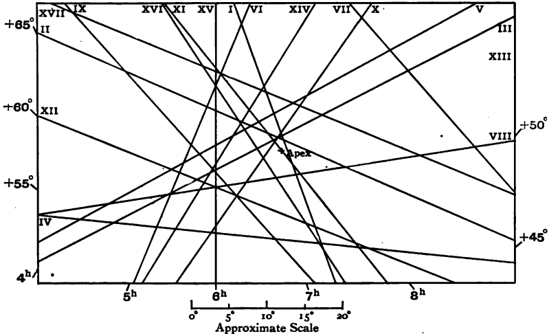
FIG. 11.—Convergence of the Directions of Drift II. from the 17 Regions.
